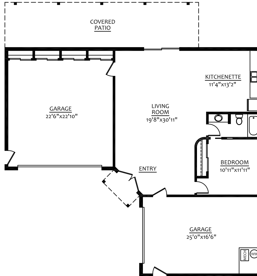
GUEST HOUSE AND GARAGES
